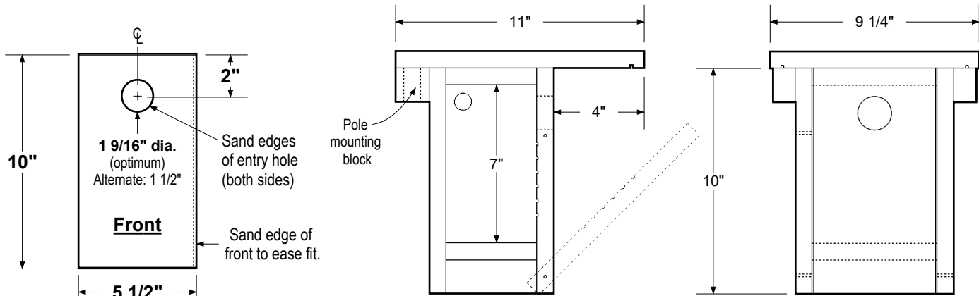
Front View
